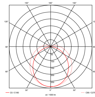
FERAX-24W-N-5000K light spread
